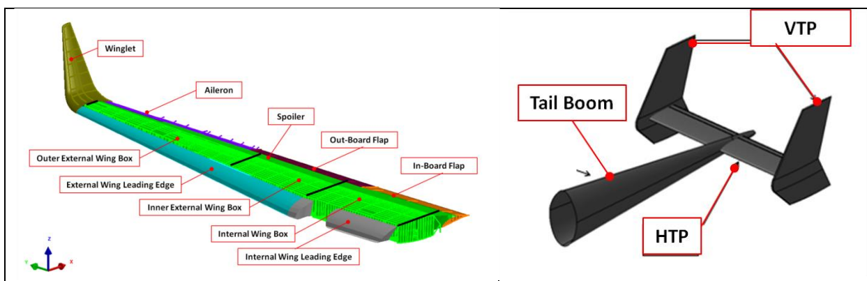
Figure 2. Structural components of the Regional Aircraft FTB2 wing –upper-& the LifeRCraft tail unit
