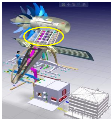
Fig. 3: Scetch of the structure and system integration of the CROR-demo engine to the flying test bed and the structural part to be developed in Module B (Pylon marget in yellow)
