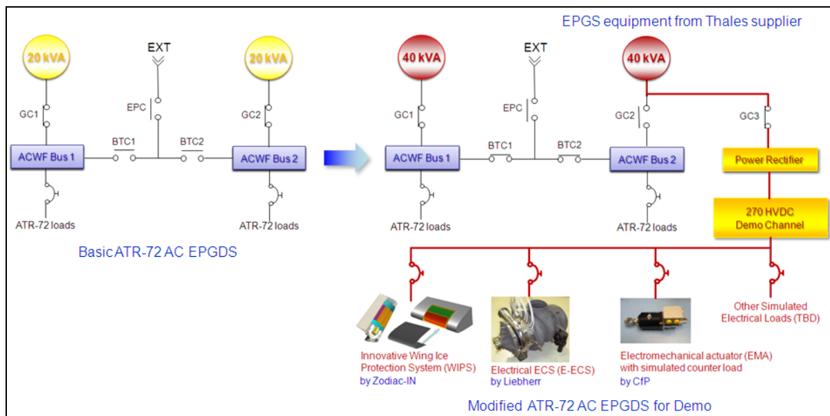
ATR-72 EPDS modification with demo loads for in-flight testing objectives
