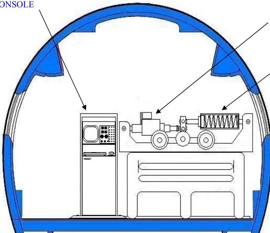
Fig. 1 – Installation concept drawing of EMA, ECU and their Test Bench on the demonstrator airplane.
