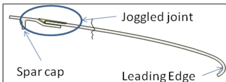
Figure 1: Joggled joint
