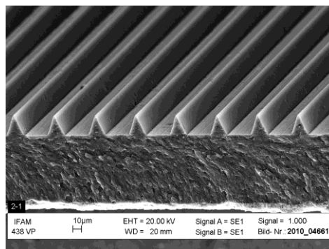
Figure 3: Scanning Electron Microscope of the painted Riblet-structure on metal substrate
