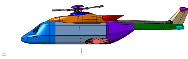
GRC common helicopter platform derived from the GOAHEAD wind-tunnel model
