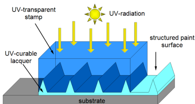
Figure 1: Application and curing of riblet painting through the silicone matrix
